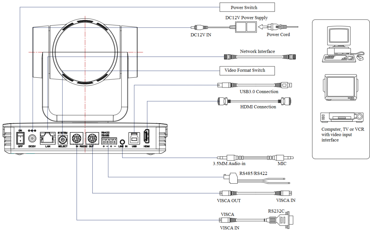
Figure 1.3 Wiring Diagram
