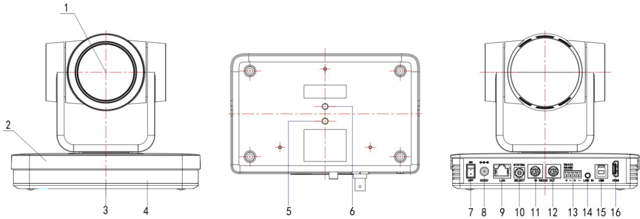
Figure 1.1 Product Interface
