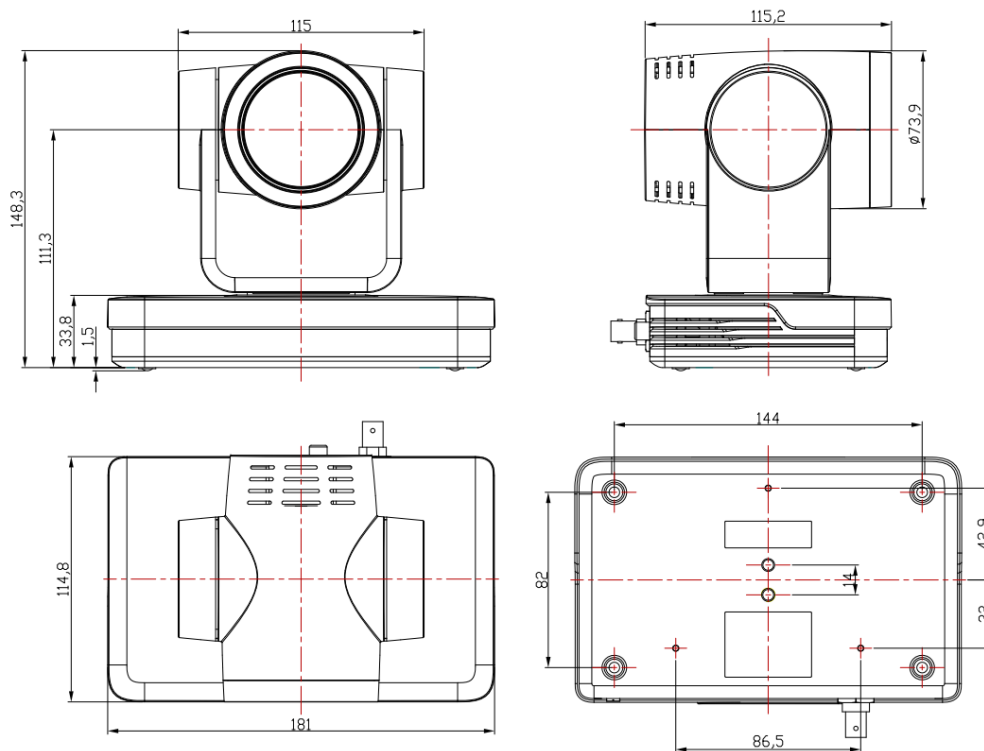
Figure 2.2 Product Dimension
